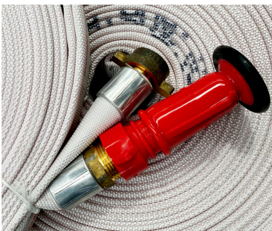
Crimped coupling & nozzle
